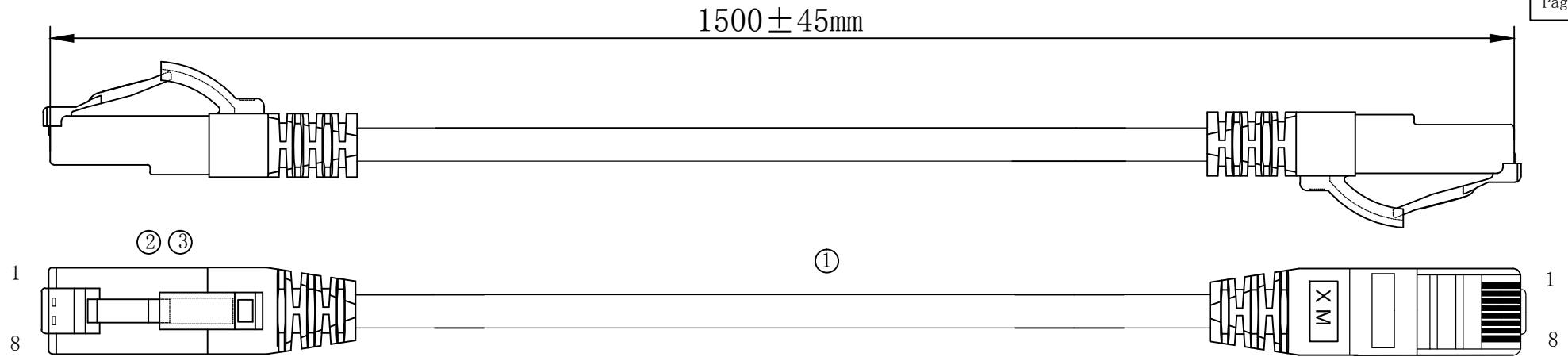
WIRING DIAGRAM(568B)
