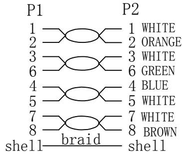
WIRING DIAGRAM(568B)
