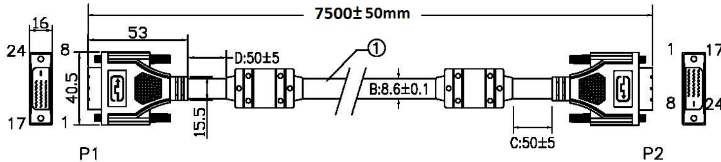
DVI Male (DVI-D, dual link)
